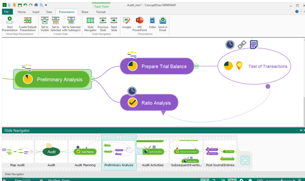
Figure 7: Slide Navigator
