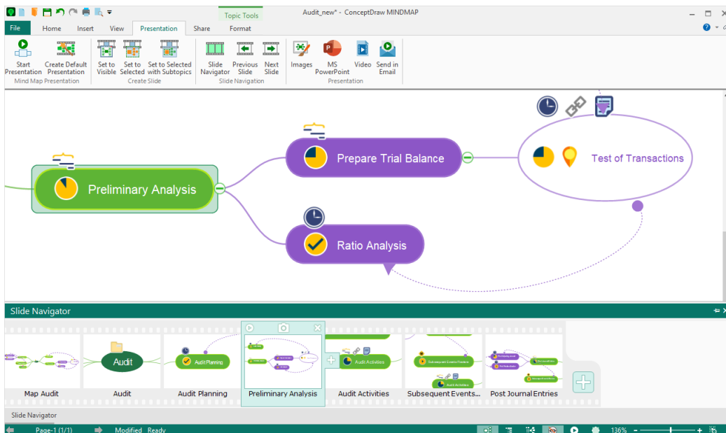
Figure 7: Slide Navigator
