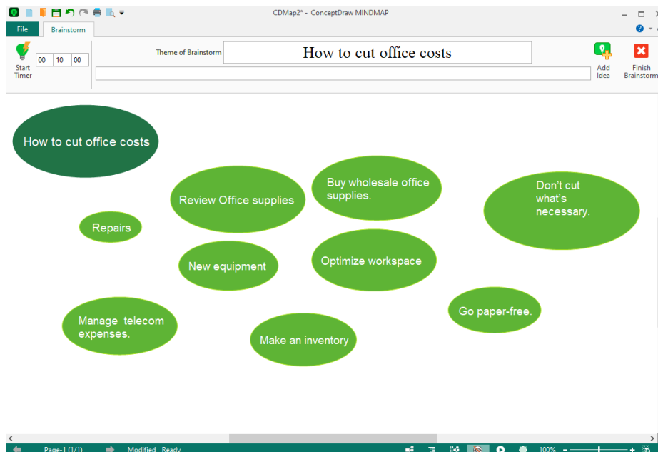
Figure 8: Brainstorm mode
