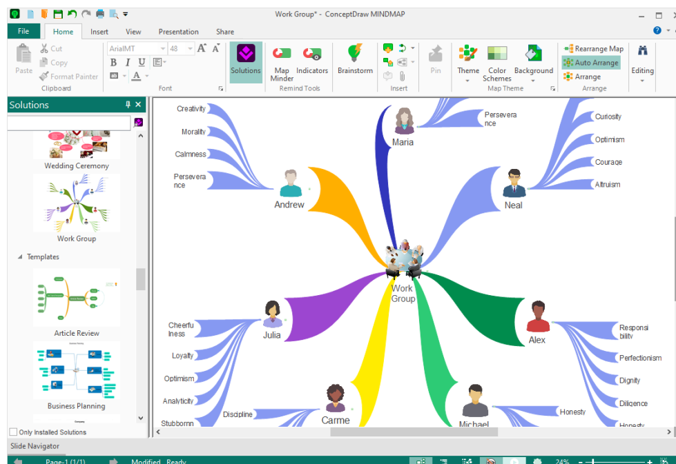
Figure 9: Solutions Panel
