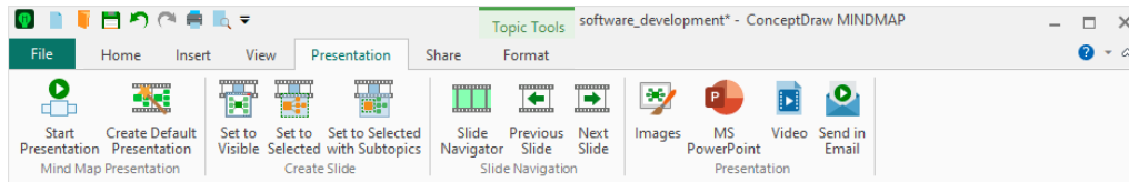
Figure 6: Presentation toolbar
