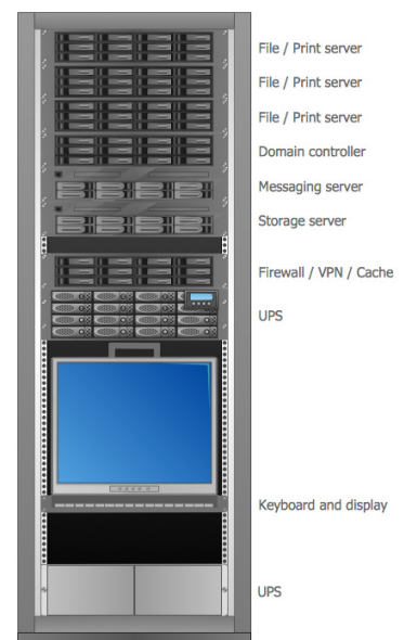
Sample of a Rack Diagram created using ConceptDraw PRO enhanced with Rack Diagrams solution from ConceptDraw Solution Park.
