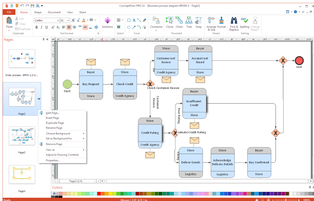
Figure 12: Page Navigator
