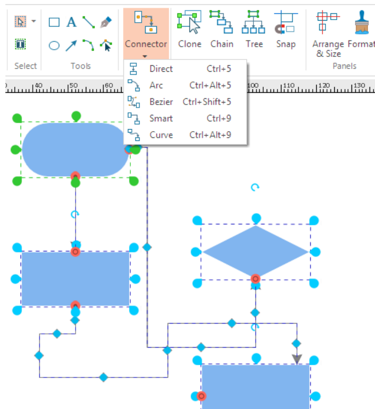
Figure 5: Connectors
