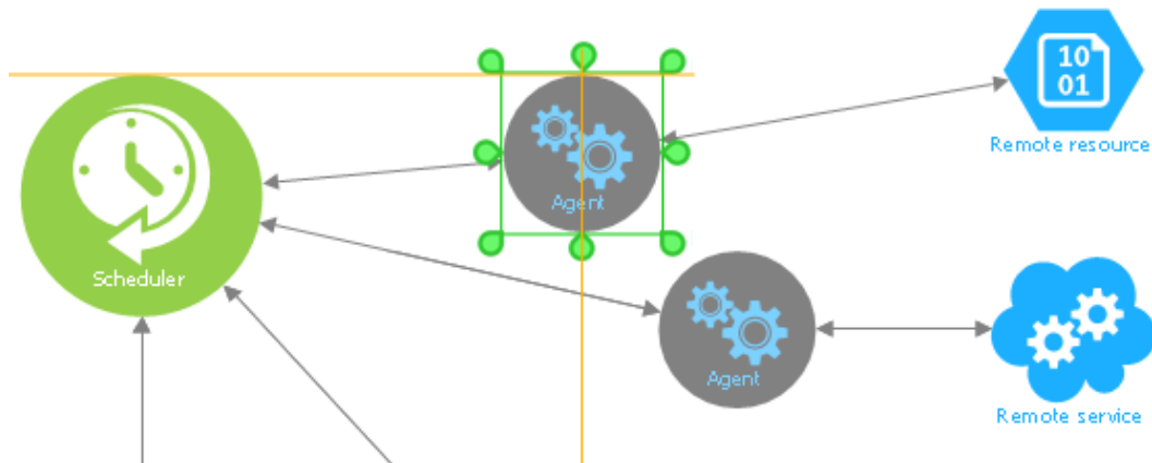
Figure 4: Adding Shapes
