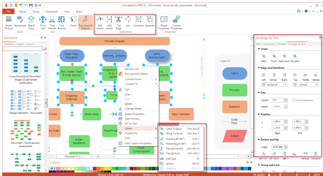
Figure 7: Shape tools
