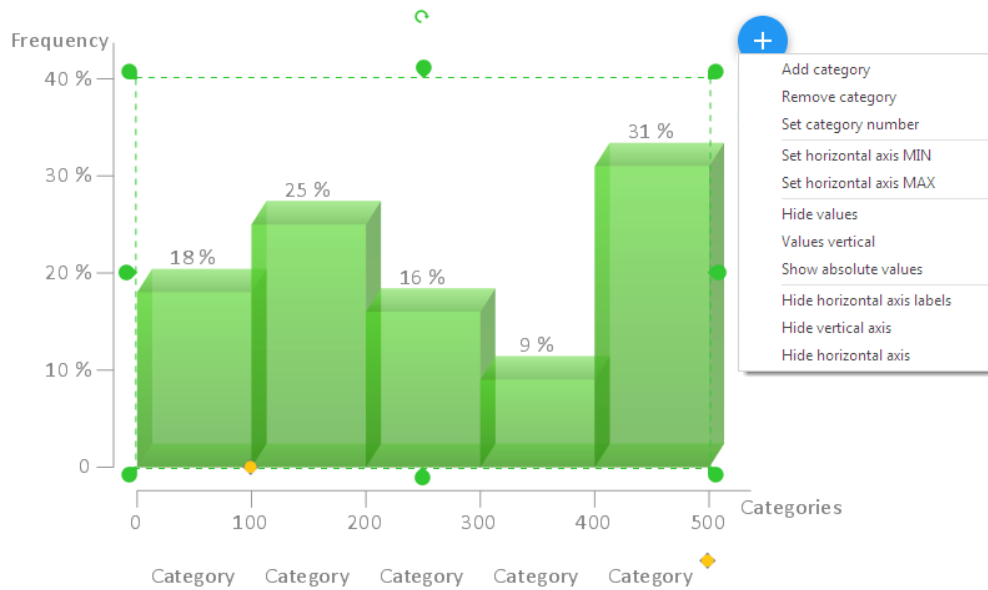
Figure 10: Smart object
